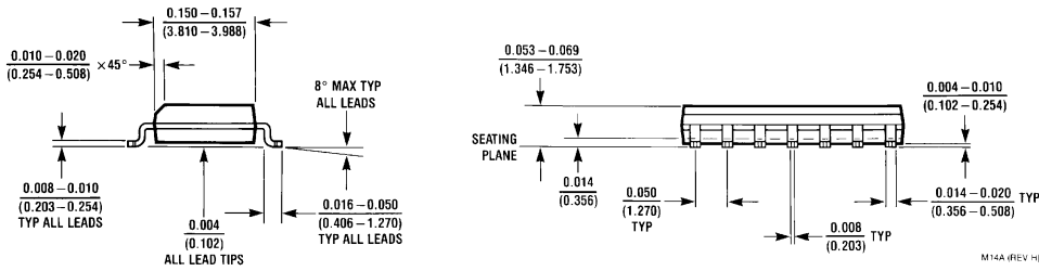
14-Lead Small Outline Molded Package (M) Order Number DM74LS74AM NS Package Number M14A
