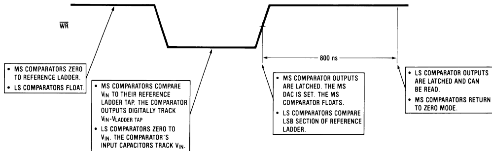
FIGURE 11. Operating Sequence (WR-RD Mode)
