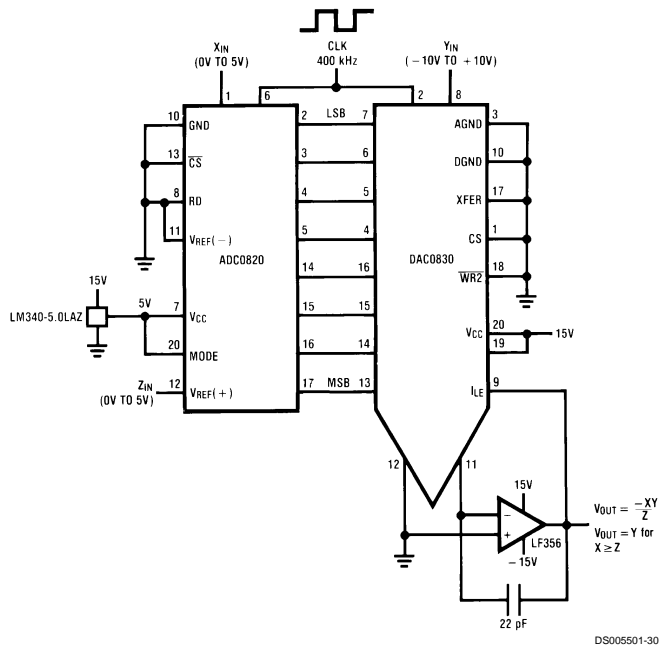
8-Bit 2-Quadrant Analog Multiplier
