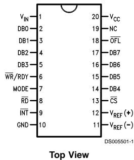
Dual-In-Line, Small Outline and SSOP Packages
