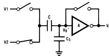
FIGURE 6. Sampled-Data Comparator
