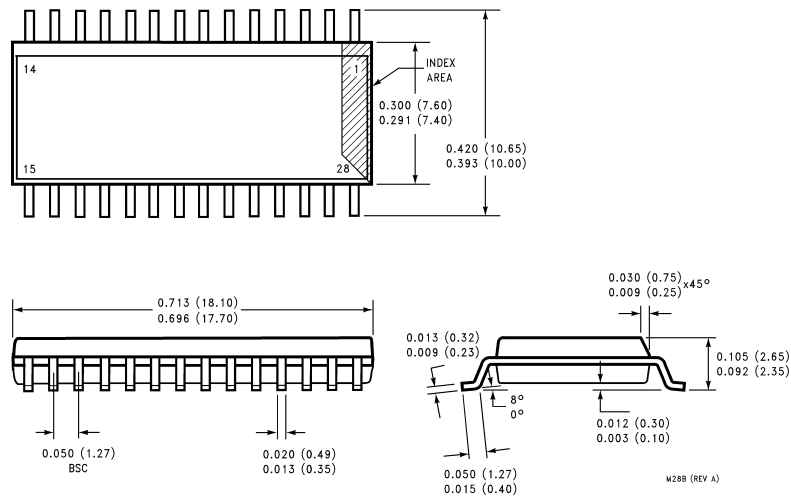
Order Number ADC10664CIWM NS Package Number M28B
