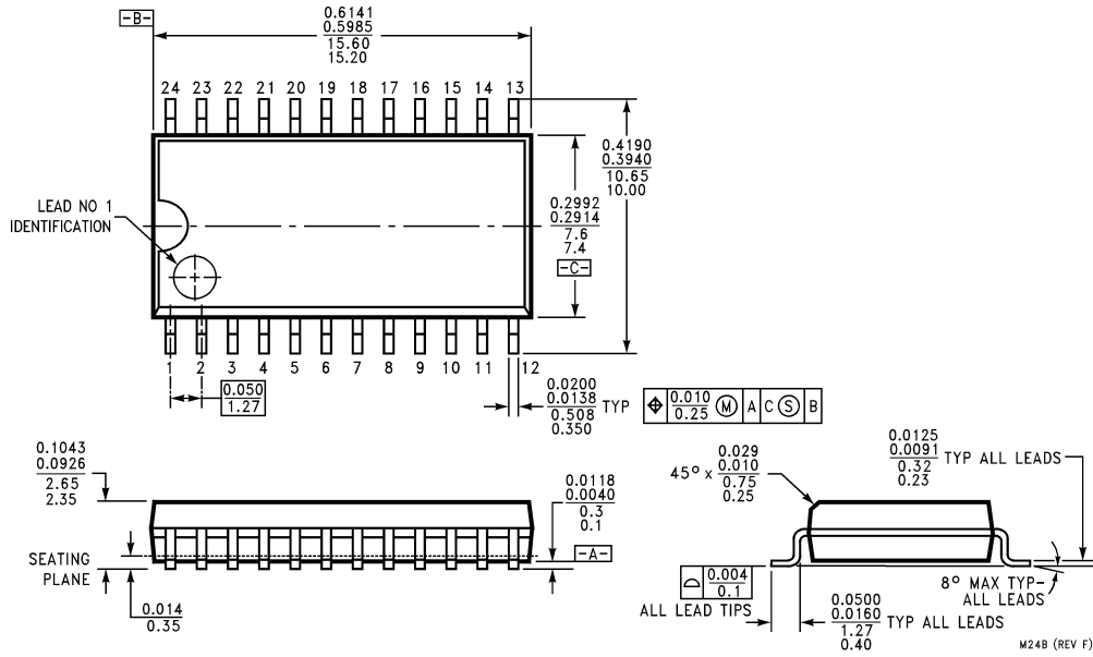
Order Number ADC10662CIWM NS Package Number M24B
