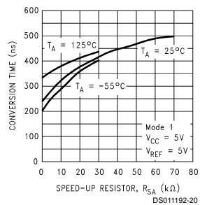
Conversion Time vs Speed-Up Resistor
