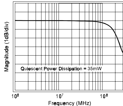
Frequency Response for \pm 5V
