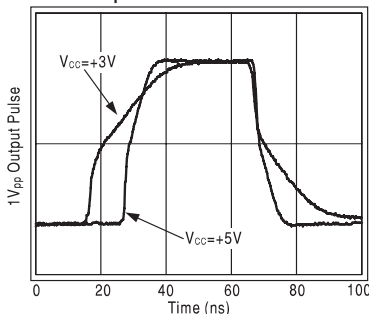
Pulse Response
