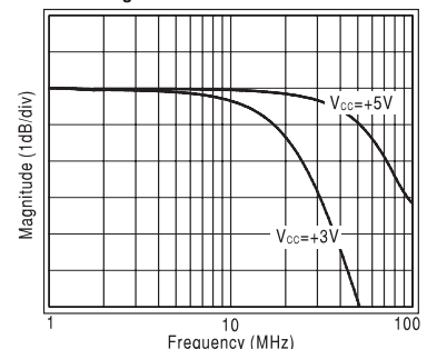
Small-Signal Bandwidth
