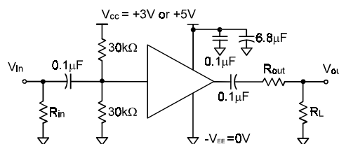
Single-Supply Circuit
