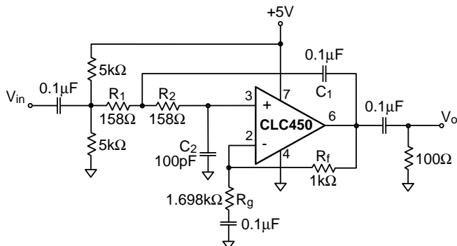
Figure 9: Lowpass Filter Topology
