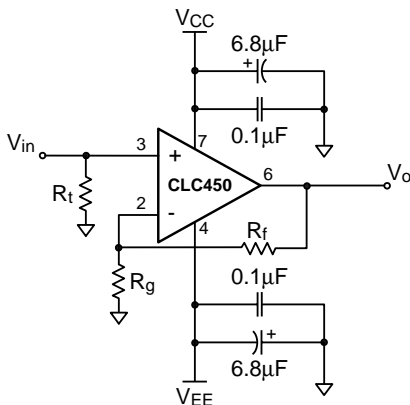
Figure 5: Dual Supply Non-Inverting Configuration
