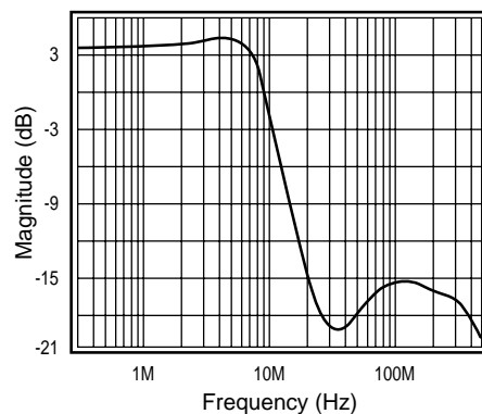
Figure 11: Lowpass Response
