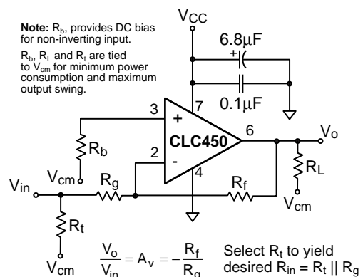
Figure 2: Inverting Configuration
