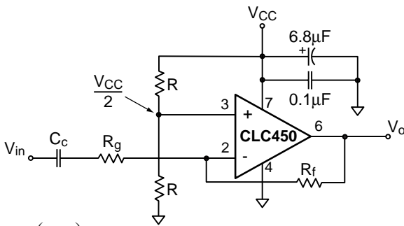
Figure 3: AC Coupled Non-Inverting Configuration
