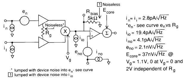
Figure 4: CLC520 Noise Model
