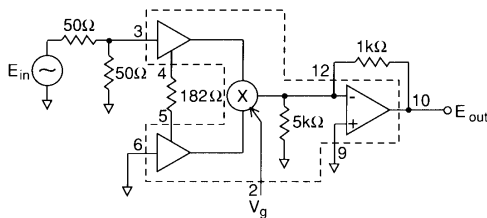
Figure 6: Typical Circuit
