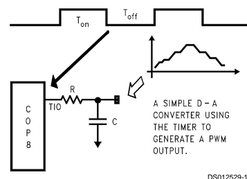
FIGURE 10. Timer Application
