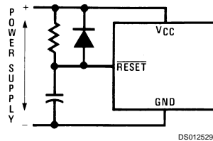
FIGURE 4. Recommended Reset Circuit
