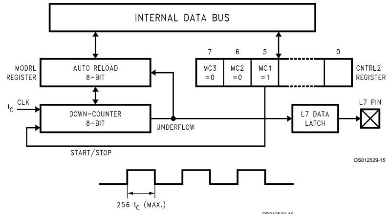
FIGURE 13. Mode 2a: 50% Duty Cycle Output
