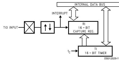
FIGURE 9. Timer Capture Mode Block Diagram
