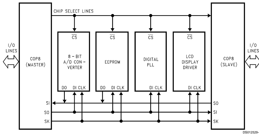
FIGURE 7. MICROWIRE/PLUS Application
