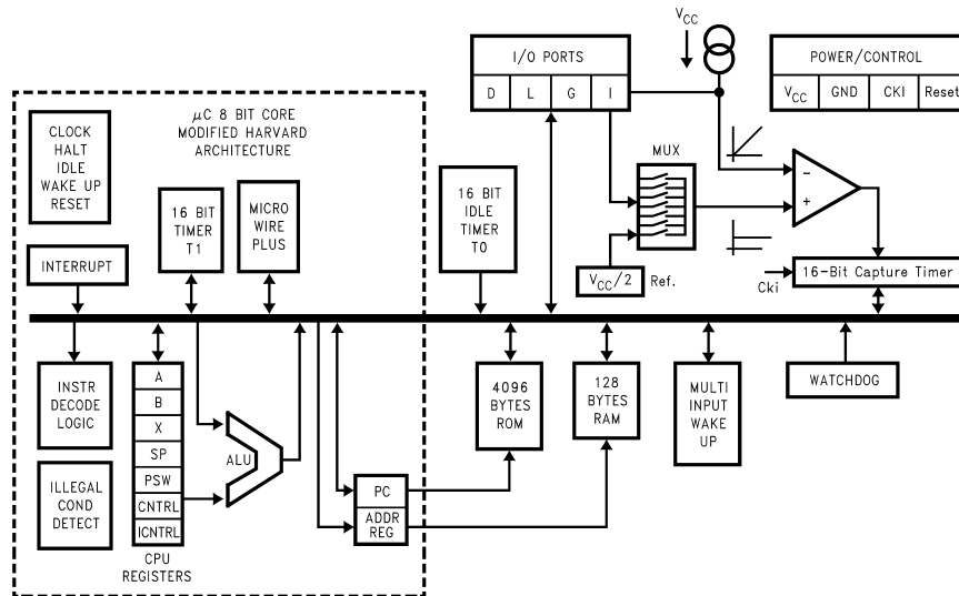
FIGURE 1. Block Diagram
