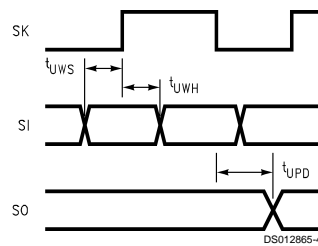
FIGURE 4. MICROWIRE/PLUS Timing
