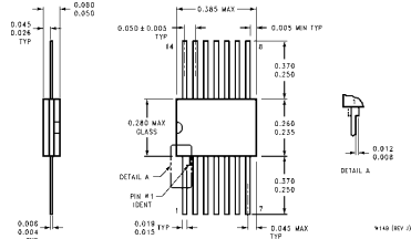
14-Lead Ceramic Flat Package (W) Order Number DM5407W NS Package Number W14B
