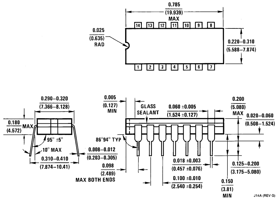
14-Lead Ceramic Dual-In-Line Package (J) Order Number DM54L10J NS Package Number J14A
