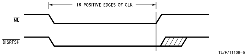
FIGURE 5a. Chip Reset but Not Programmed
