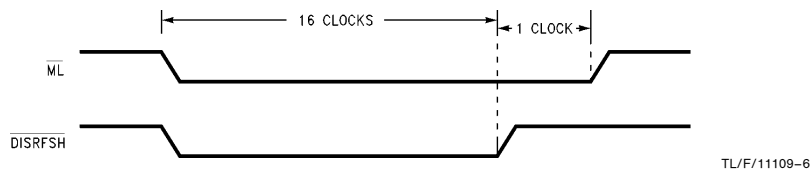
FIGURE 5b. Chip Reset and Programmed
