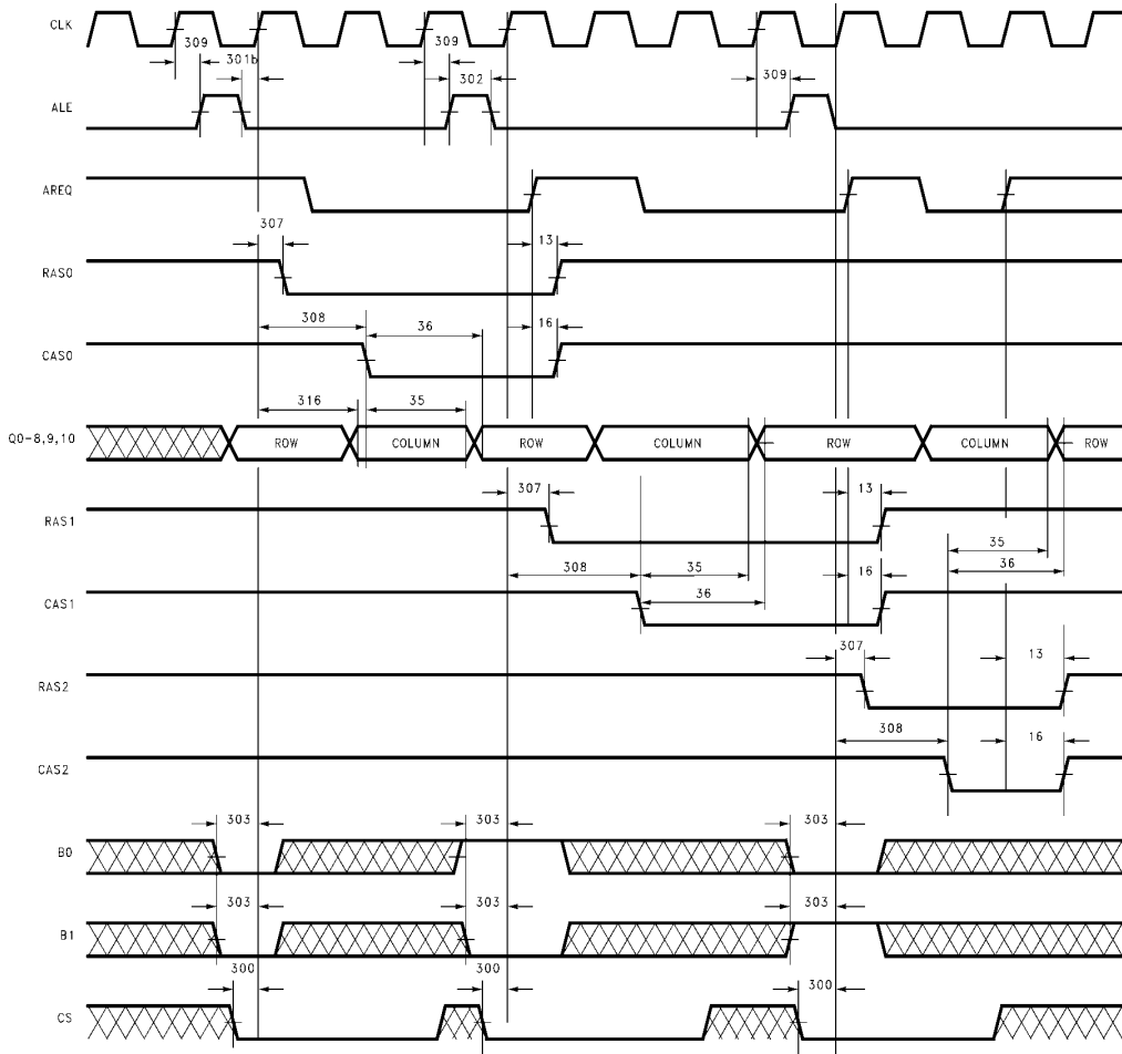
FIGURE 41. 300: Mode 0 Interleaving
