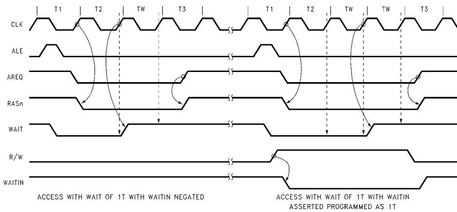
FIGURE 24b. \overline{\text{WAITIN}} Example ( \overline{\text{WAIT}} is Sampled at the End of "T2").
