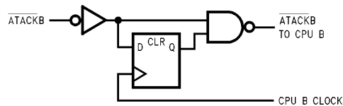
FIGURE 33c. Modifying Wait Logic for Port B
