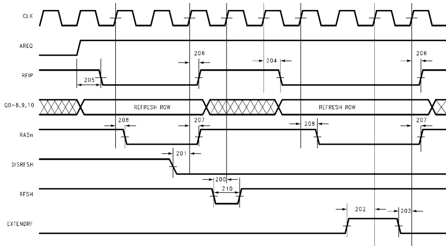
FIGURE 39. 200: Refresh Timing
