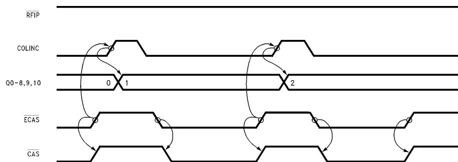
FIGURE 10. Column Increment
