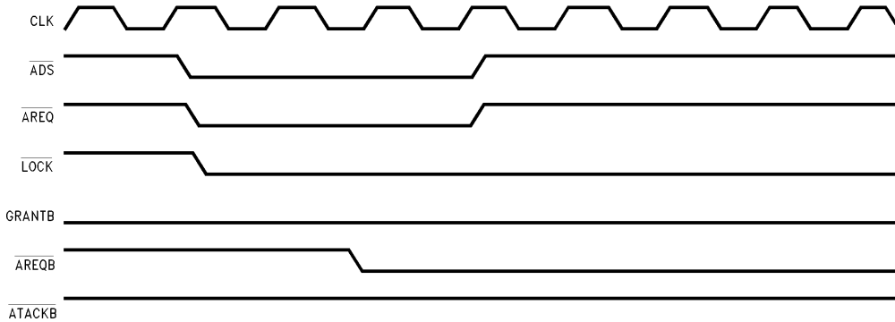
FIGURE 35. \overline{\text{LOCK}} Function
