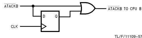
FIGURE 33b. Delayed Port B Access
