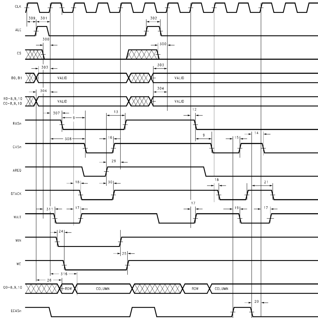
FIGURE 40. 300: Mode 0 Timing
