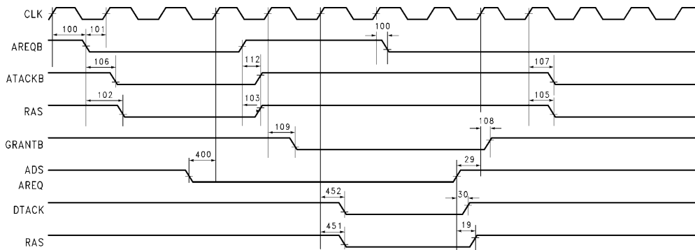
FIGURE 38. 100: Port A and Port B Dual Access
