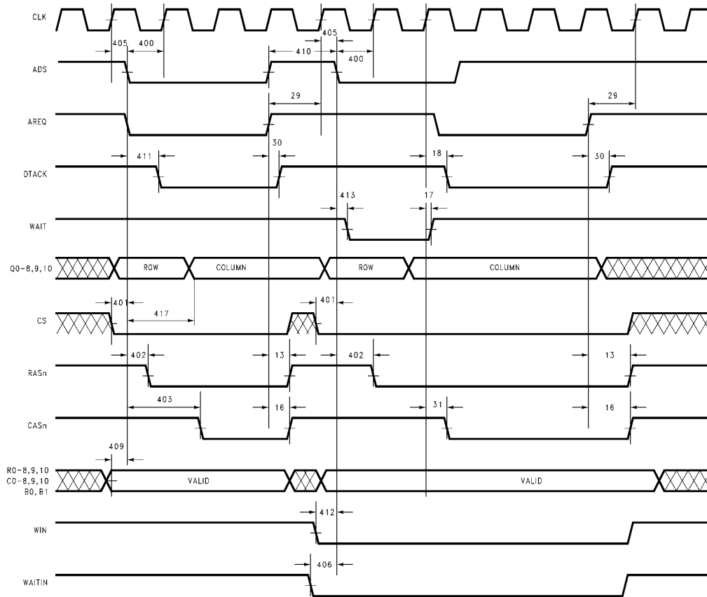
FIGURE 42. 400: Mode 1 Timing
