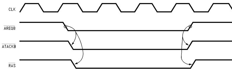
FIGURE 33a. Non-Delayed Port B Access
