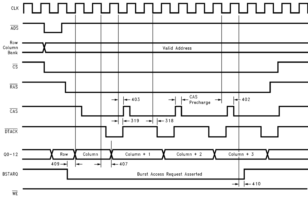
FIGURE 12. Burst Read Access
