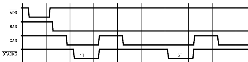
FIGURE 23d. 1T during Opening, 3T during Burst
