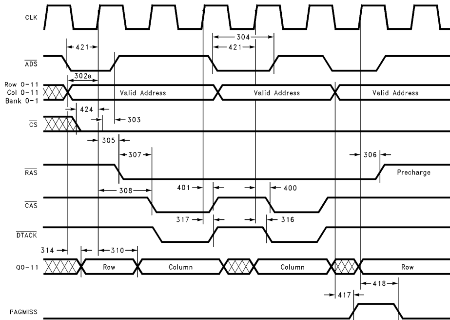
FIGURE 8. Opening Access Followed by Page Accesses
