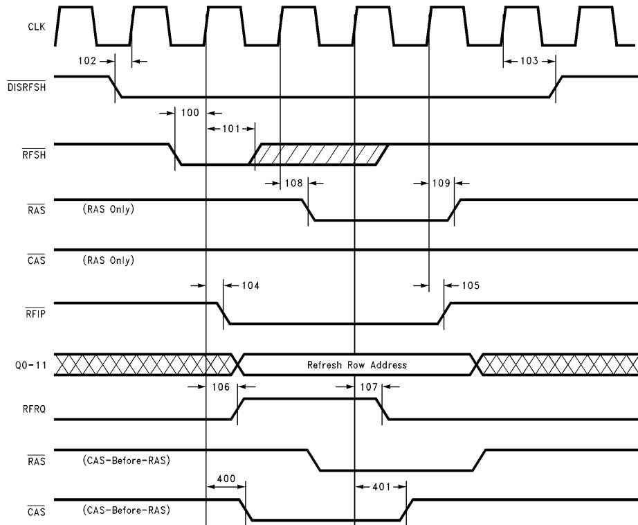
FIGURE 26. Refresh Timing
