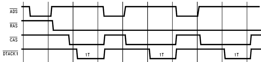
FIGURE 22b. \overline{DTACK} is Programmed 1T for Openings and 1T during Page
