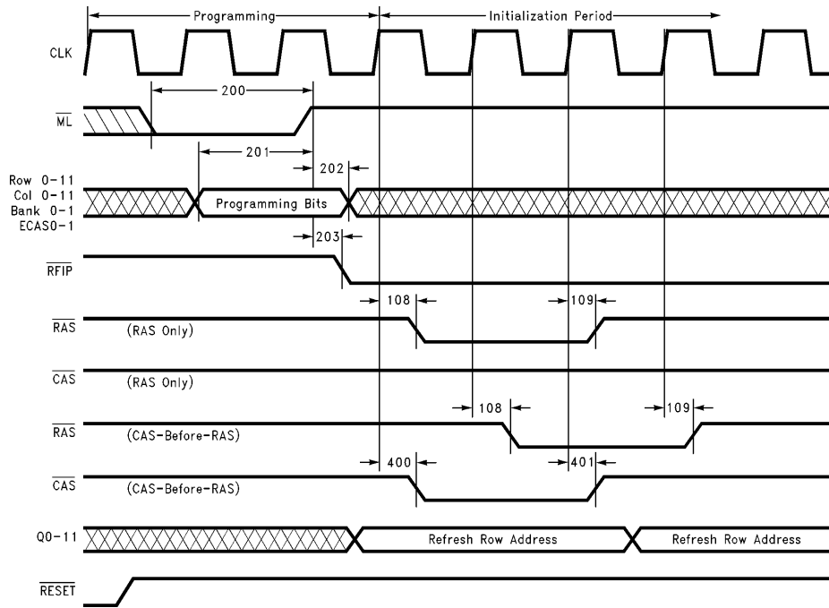
FIGURE 28. Programming and Initialization Period Timing
