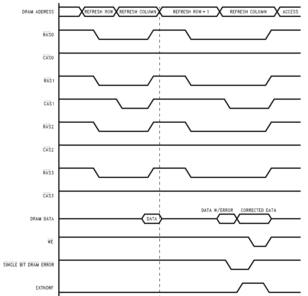
FIGURE 16. Error Scrubbing during Refresh (Two Refresh Cycles Shown)
