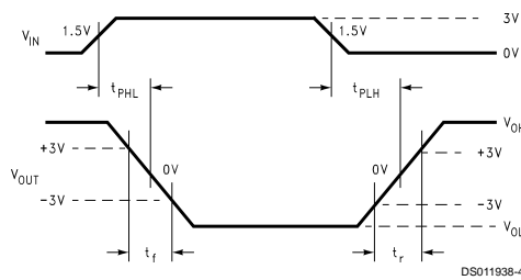
FIGURE 2. Driver Propagation Delay and Transition Time Waveforms Slew Rate (SR) = 6V/(tr or tr)
