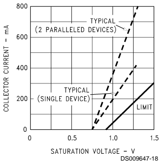
Collector Current vs Saturation Voltage
