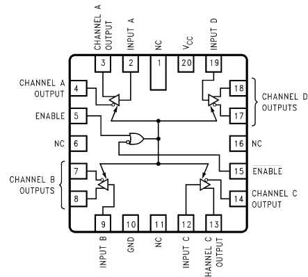
20-Lead Ceramic Leadless Chip Carrier (E)
