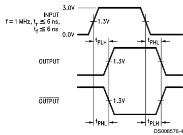
FIGURE 2. Propagation Delays
