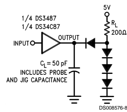
FIGURE 5. Propagation Delays Test Circuit for "LS-Type" Load
