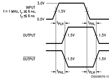
FIGURE 8. Load Propagation Delays for "LS-Type" Load
