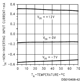
Receiver Non-Inverting Input Current vs Temperature
