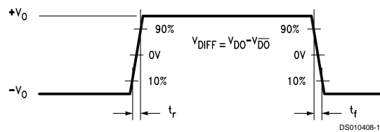
FIGURE 8. Driver Differential Transition Timing
