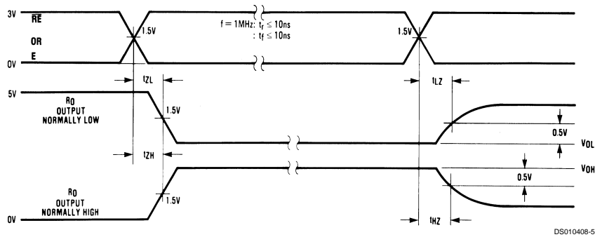
FIGURE 4. Receiver Enable/Disable Propagation Delay Timing
