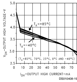
Driver V_{OH} vs I_{OH} vs Temperature
