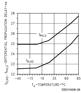
Receiver Differential Propagation Delay vs Temperature
