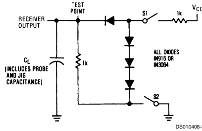
FIGURE 2. Receiver Propagation Delay Test Circuit
