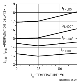
Driver Single-Ended Propagation Delay vs Temperature
