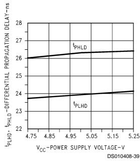
Receiver Differential Propagation Delay vs V_{CC}
