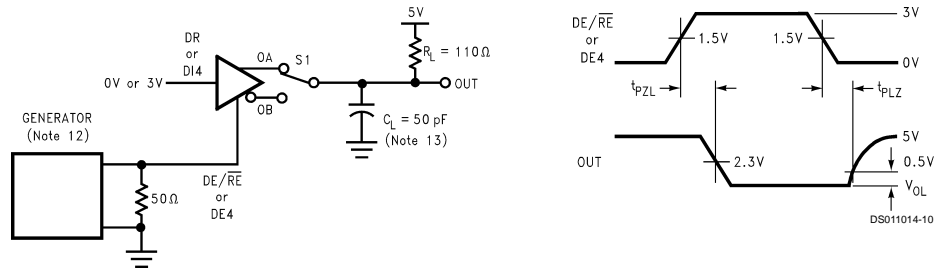
FIGURE 6. Driver Enable and Disable Timing ( t_{PZL} , t_{PLZ} )
