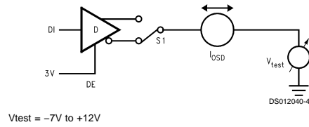
FIGURE 4. Driver I_{ODS}
