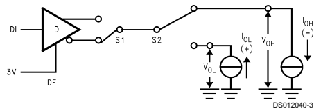
FIGURE 3. Driver V_{OH} and V_{OL}
