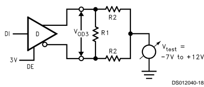
FIGURE 2. Driver V_{OD3}
