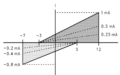
FIGURE 18. Input Current vs Input Voltage Operating Range
