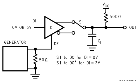
FIGURE 9. TRI-STATE Test Circuit ( t_{PLZ} , t_{PLZ} )
