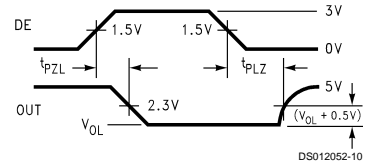
FIGURE 10. TRI-STATE Waveforms ( t_{PLZ} , t_{PLZ} )
