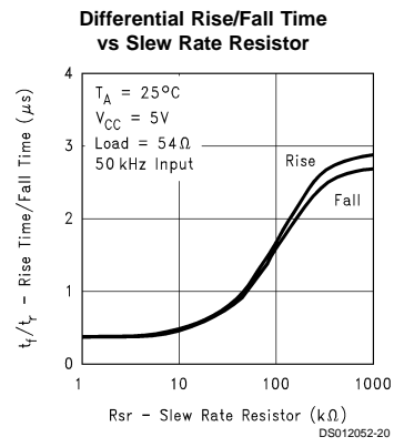
FIGURE 19. Slew Rate Resistor vs Rise/Fall Time
