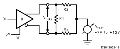
FIGURE 2. Driver V_{OD3}
