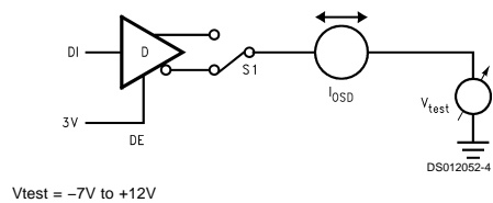
FIGURE 4. Driver I_{0SD}
