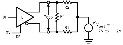
FIGURE 5. V_{OD3}
