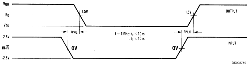
FIGURE 7. Receiver Propagation Delays
