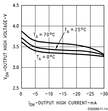
Driver V_{OH} vs I_{OH} vs Temperature
