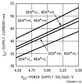
Supply Current vs V_{CC}
