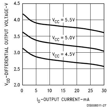
Driver V OD vs V CC
