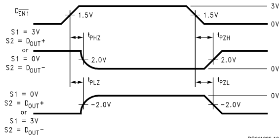
FIGURE 8. Differential Driver TRI-STATE Waveforms
