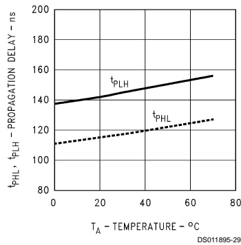
Driver Propagation Delay vs Temperature
