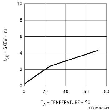
Receiver Output Skew vs Temperature
