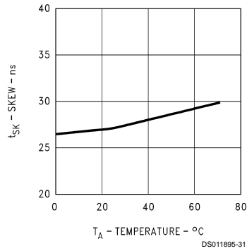
Driver Skew vs Temperature
