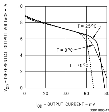
Differential Driver Output Voltage vs Output Current
