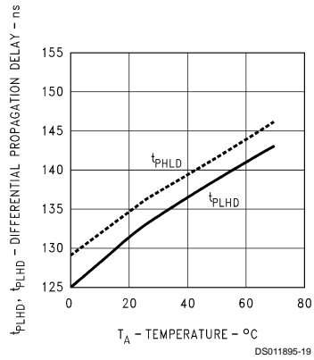
Differential Driver Propagation Delay vs Temperature
