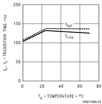
Differential Transition Time vs Temperature
