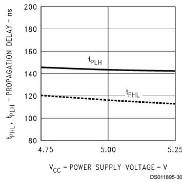
Driver Propagation Delay vs Power Supply Voltage
