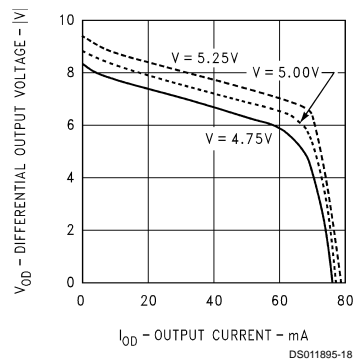
Differential Driver Output Voltage vs Output Current
