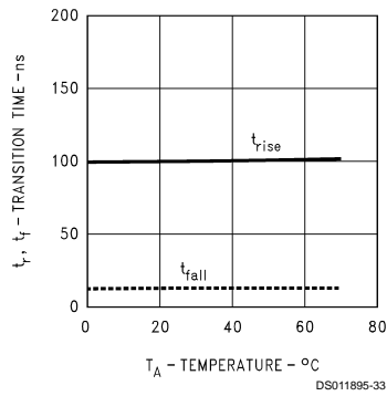
Driver Transition Time vs Temperature
