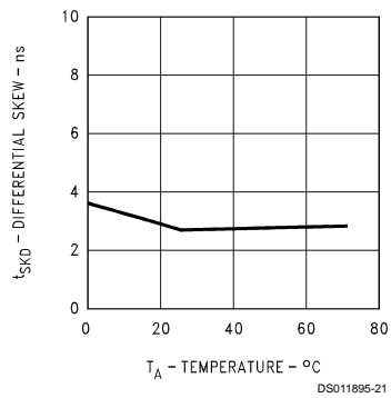
Differential Driver Skew vs Temperature
