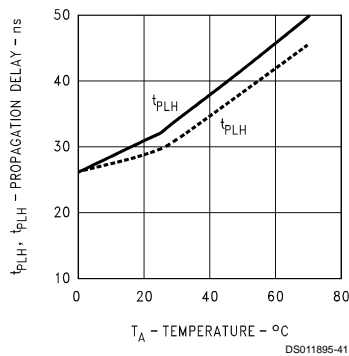
Receiver Output Propagation Delay vs Temperature
