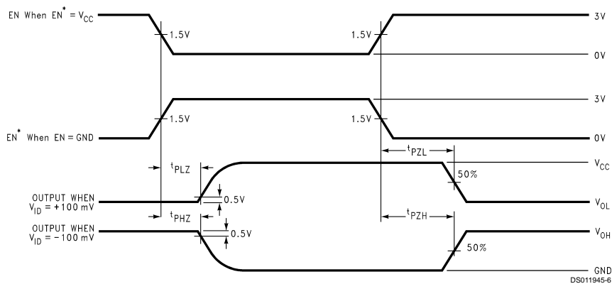
FIGURE 4. Receiver TRI-STATE Delay Waveforms
