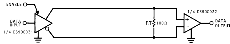
FIGURE 5. Point-to-Point Application
