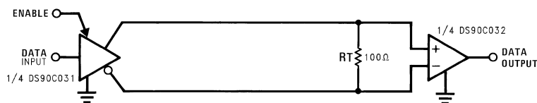
FIGURE 5. Point-to-Point Application
