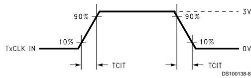
FIGURE 5. DS90C363A/DS90CF363A (Transmitter) Input Clock Transition Time
