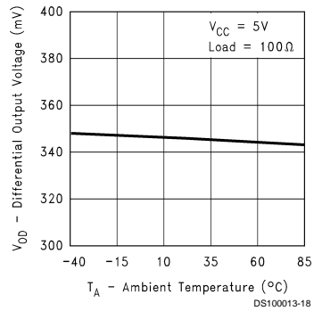
Differential Output Voltage vs Ambient Temperature
