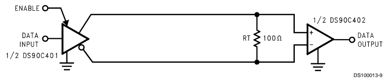
FIGURE 4. Point-to-Point Application
