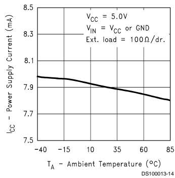
Power Supply Current vs Temperature (Ext. load = 100 \Omega /dr.)
