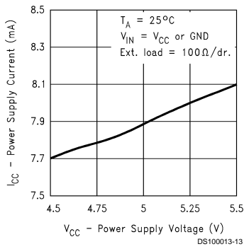
Power Supply Current vs Power Supply Voltage (Ext. load = 100 \Omega /dr.)
