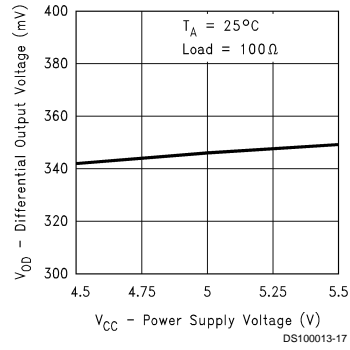
Differential Output Voltage vs Power Supply Voltage
