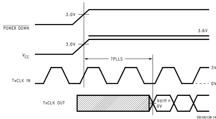
FIGURE 8. DS90C363A/DS90CF363A (Transmitter) Phase Lock Loop Set Time
