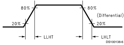
FIGURE 4. DS90C363A/DS90CF363A (Transmitter) LVDS Transition Times
