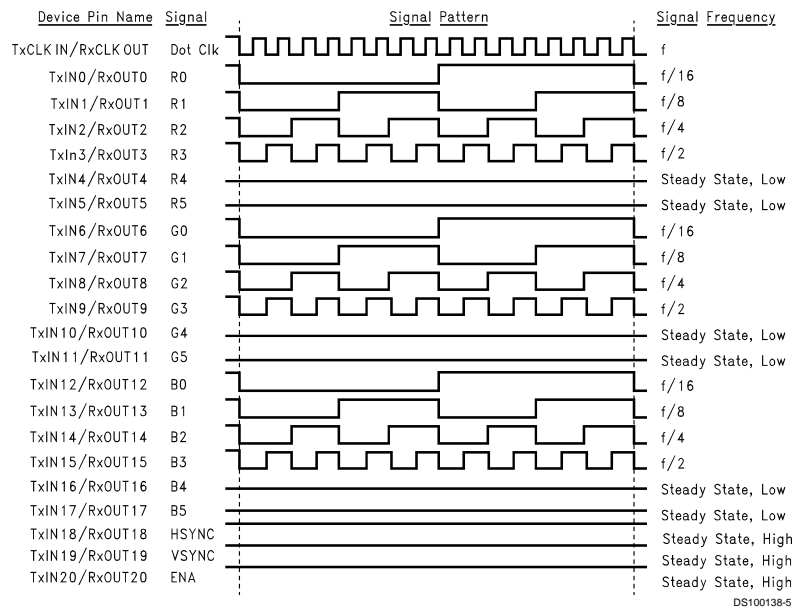
FIGURE 2. "16 Grayscale" Test Pattern (Notes 7, 8, 9, 10)
