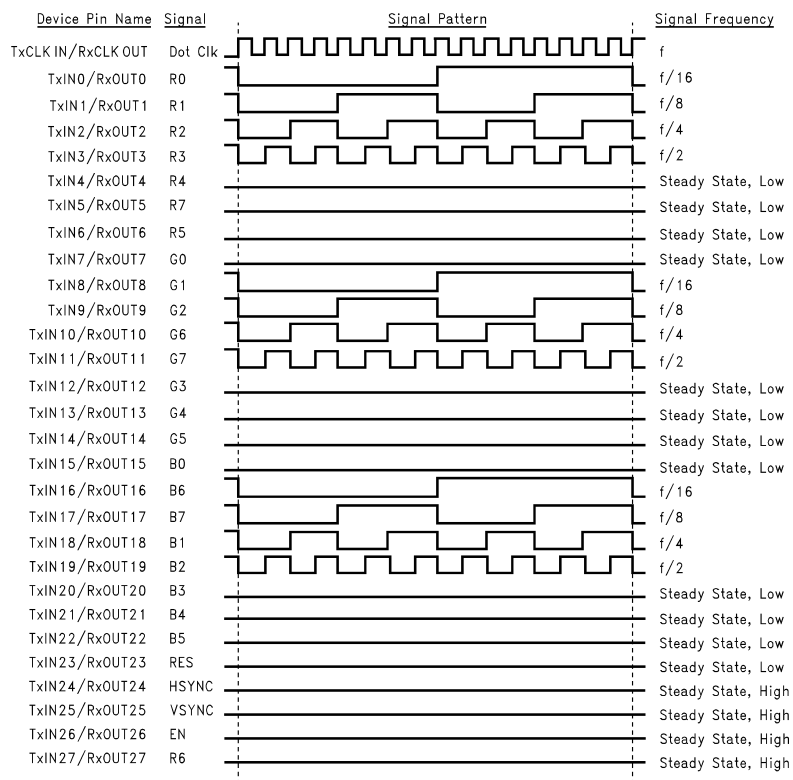
FIGURE 2. "16 Grayscale" Test Pattern (Notes 7, 8, 9, 10)
