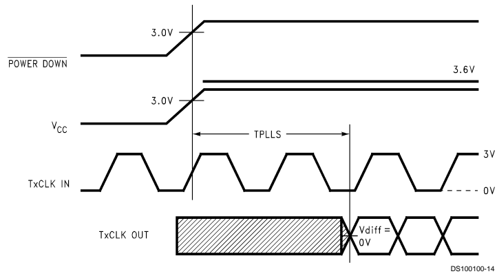
FIGURE 8. DS90C383A/DS90CF383A (Transmitter) Phase Lock Loop Set Time
