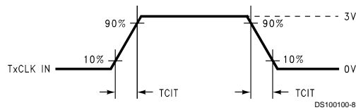
FIGURE 5. DS90C383A/DS90CF383A (Transmitter) Input Clock Transition Time
