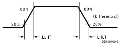
FIGURE 4. DS90C383A/DS90CF383A (Transmitter) LVDS Transition Times
