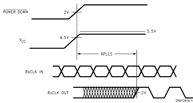
FIGURE 12. DS90CF584 (Receiver) Phase Lock Loop Set Time
