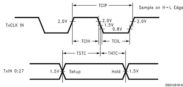
FIGURE 7. DS90CF583 (Transmitter) Setup/Hold and High/Low Times
