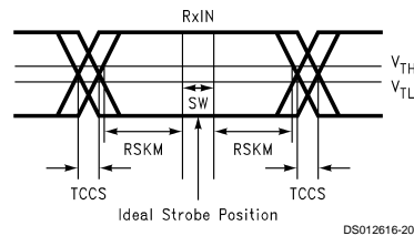
FIGURE 13. Receiver LVDS Input Pulse Position Measurement
