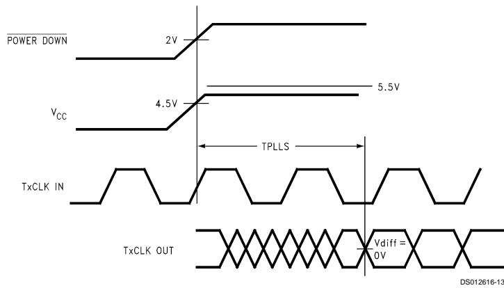
FIGURE 11. DS90CF583 (Transmitter) Phase Lock Loop Set Time
