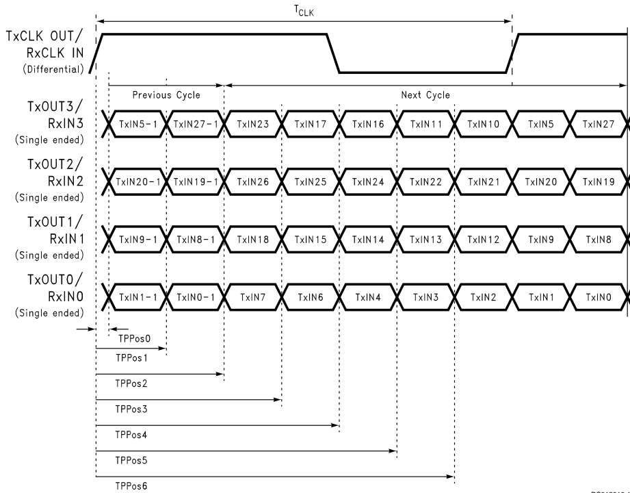
FIGURE 13. Receiver LVDS Input Pulse Position Measurement
