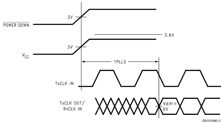
FIGURE 10. DS90CR217 (Transmitter) Phase Lock Loop Set Time
