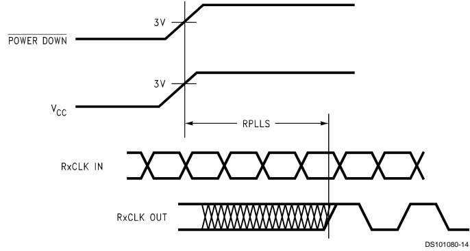
FIGURE 11. DS90CR218A (Receiver) Phase Lock Loop Set Time
