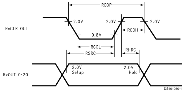
FIGURE 7. DS90CR218A (Receiver) Setup/Hold and High/Low Times
