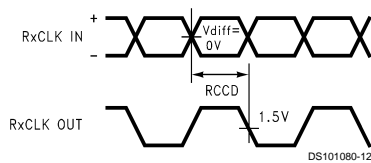
FIGURE 9. DS90CR218A (Receiver) Clock In to Clock Out Delay
