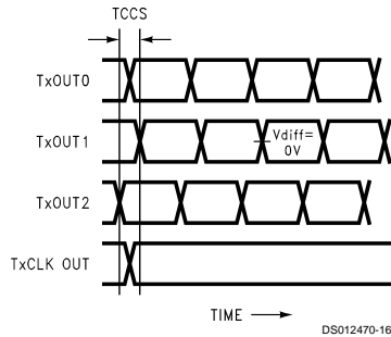
FIGURE 6. DS90CR561 (Transmitter) Channel-to-Channel Skew and Pulse Width
