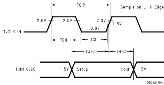
FIGURE 7. DS90CR561 Setup/Hold and High/Low Times
