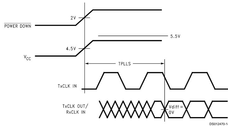
FIGURE 11. DS90CR561 (Transmitter) Phase Lock Loop Set Time
