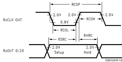
FIGURE 8. DS90CR562 Setup/Hold and High/Low Times
