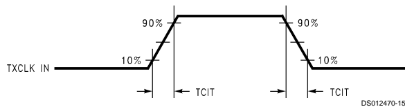
FIGURE 5. DS90CR561 (Transmitter) Input Clock Transition Time
