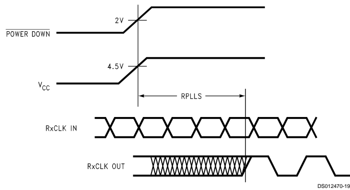
FIGURE 12. DS90CR562 (Receiver) Phase Lock Loop Set Time
