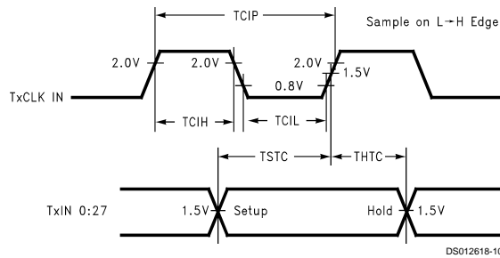
FIGURE 7. DS90CR583 (Transmitter) Setup/Hold and High/Low Times
