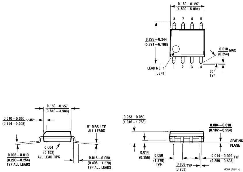
Order Number DS90LV017ATM NS Package Number M08A
