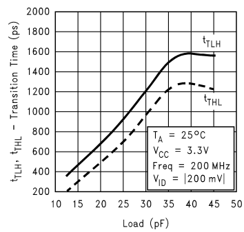
Transition Time vs Load
