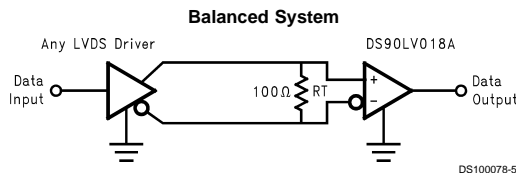
FIGURE 3. Point-to-Point Application
