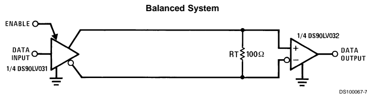
FIGURE 5. Point-to-Point Application
