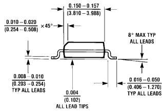
16-Lead (0.150" Wide) Molded Small Outline Package, JEDEC Order Number DS90LV032ATM NS Package Number M16A
