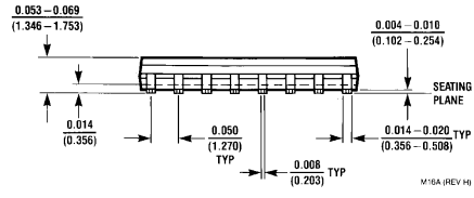
16-Lead (0.150" Wide) Molded Small Outline Package, JEDEC Order Number DS90LV032ATM NS Package Number M16A
