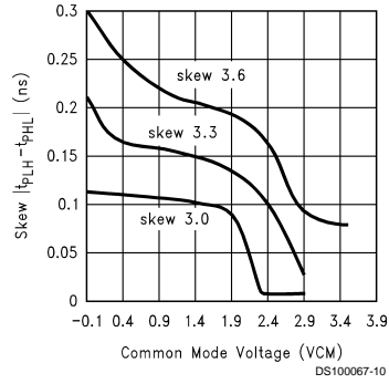
FIGURE 8. Typical Pulse Skew variation versus common-mode voltage
