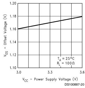
Offset Voltage vs Power Supply Voltage
