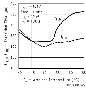
Transition Time vs Ambient Temperature
