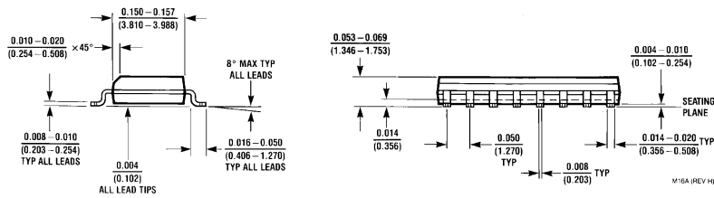
16-Lead (0.150" Wide) Molded Small Outline Package, JEDEC Order Number DS90LV047ATM NS Package Number M16A
