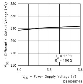
Differential Output Voltage vs Power Supply Voltage
