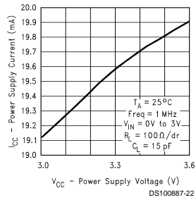
Power Supply Current vs Power Supply Voltage
