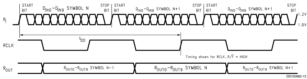
FIGURE 4. Deserializer Delay
