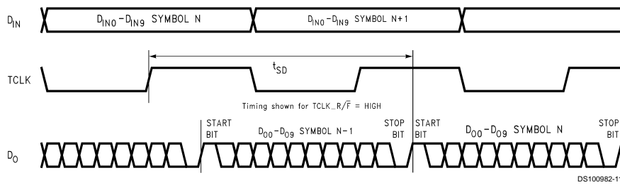
FIGURE 3. Serializer Delay
