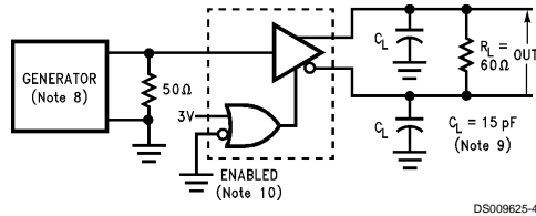
FIGURE 3. Differential Output Delay and Transition Times
