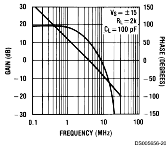
Bode Plot
