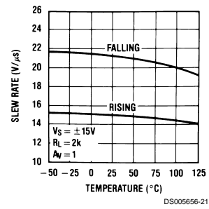
Slew Rate
