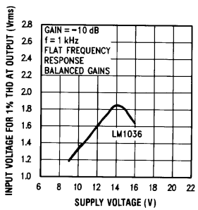
Input Signal Handling vs Supply Voltage
