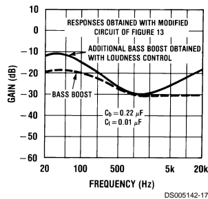
FIGURE 14. Loudness Compensated Volume Characteristic
