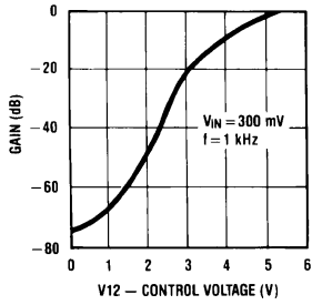
Volume Control Characteristics
