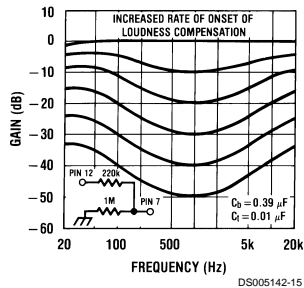
FIGURE 12. Loudness Compensated Volume Characteristic
