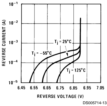
Reverse Characteristics
