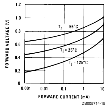
Forward Characteristics
