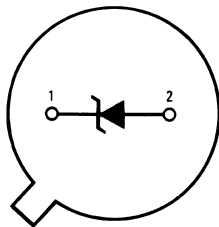
Metal Can Package (TO-46)
