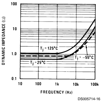
Dynamic Impedance
