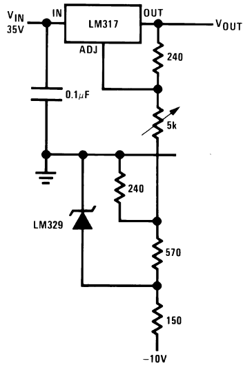
Low Cost 0–25V Regulator
