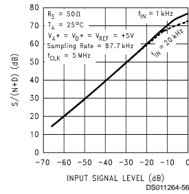
Bipolar Signal-to-Noise + Distortion Ratio vs Input Signal Level
