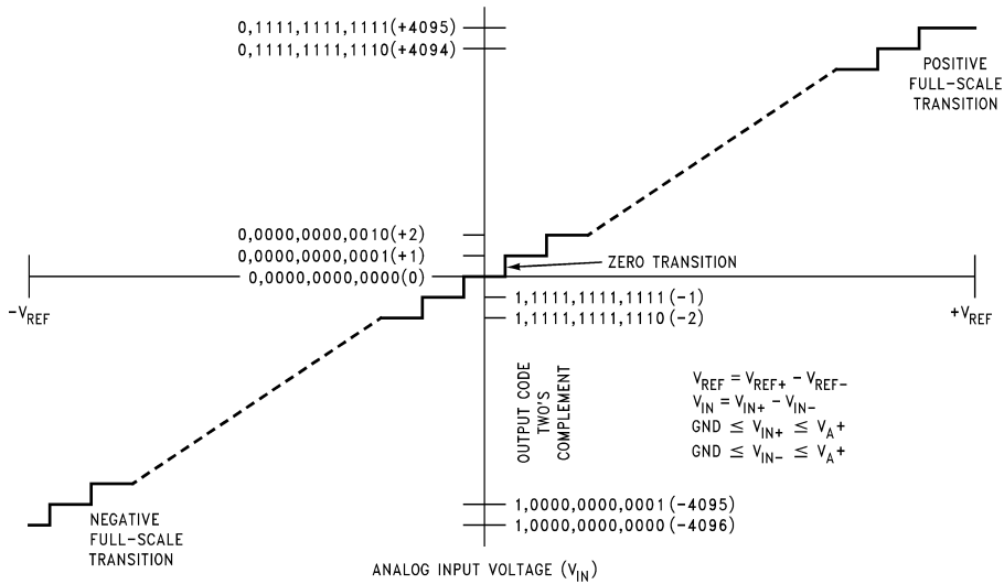
FIGURE 5. Transfer Characteristic
