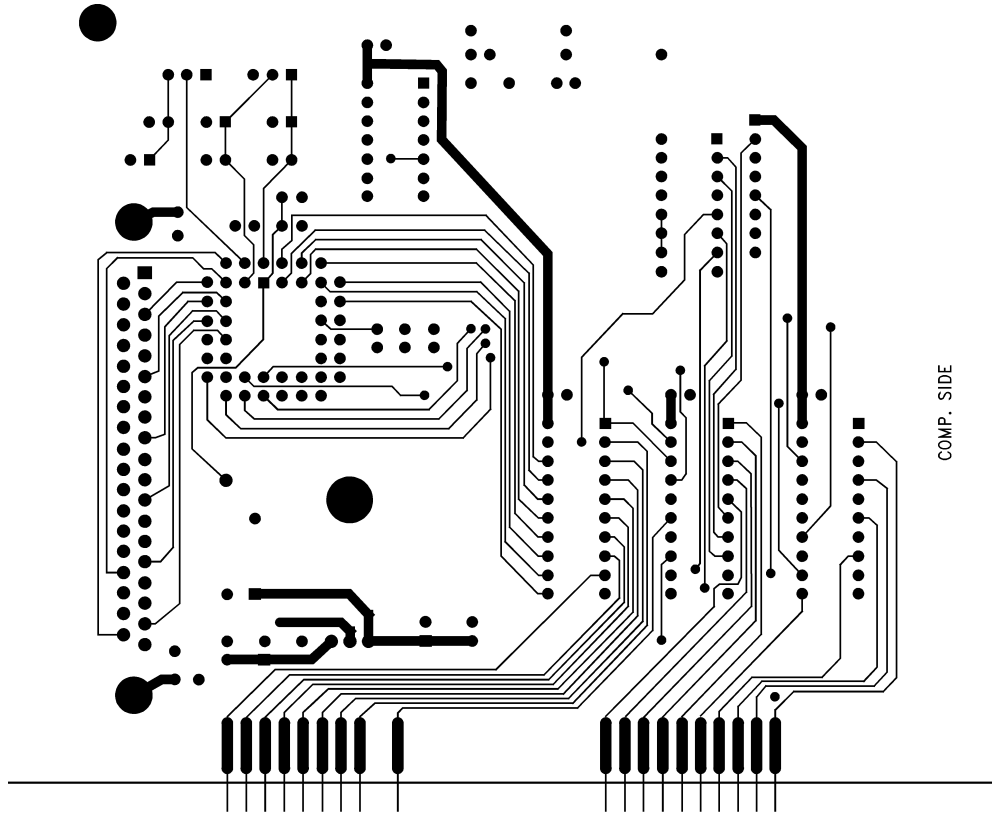
FIGURE 21. LM12(H)454/8 Evaluation/Interface Board Component-Side Layout Positive
