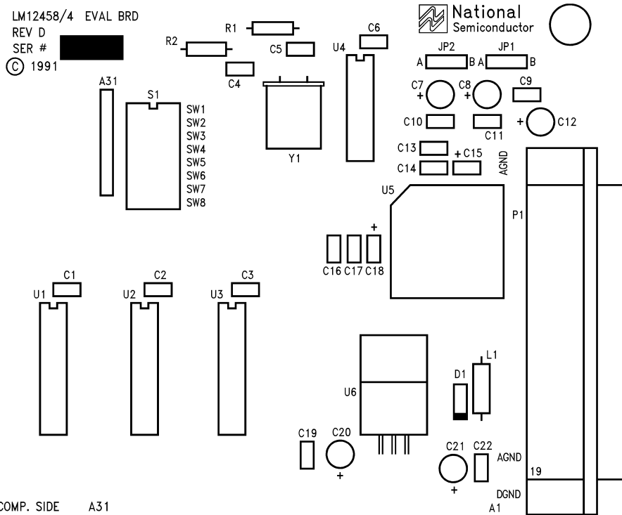
FIGURE 20. Silk-Screen Layout Showing Parts Placement on the LM12(H)454/8 Evaluation/Interface Board
