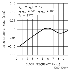
Zero Error Change vs Clock Frequency
