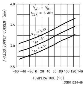
Analog Supply Current vs Temperature
