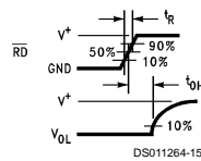
FIGURE 9. TRI-STATE Test Circuits and Waveforms
