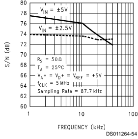
Bipolar Signal-to-Noise Ratio vs Input Frequency
