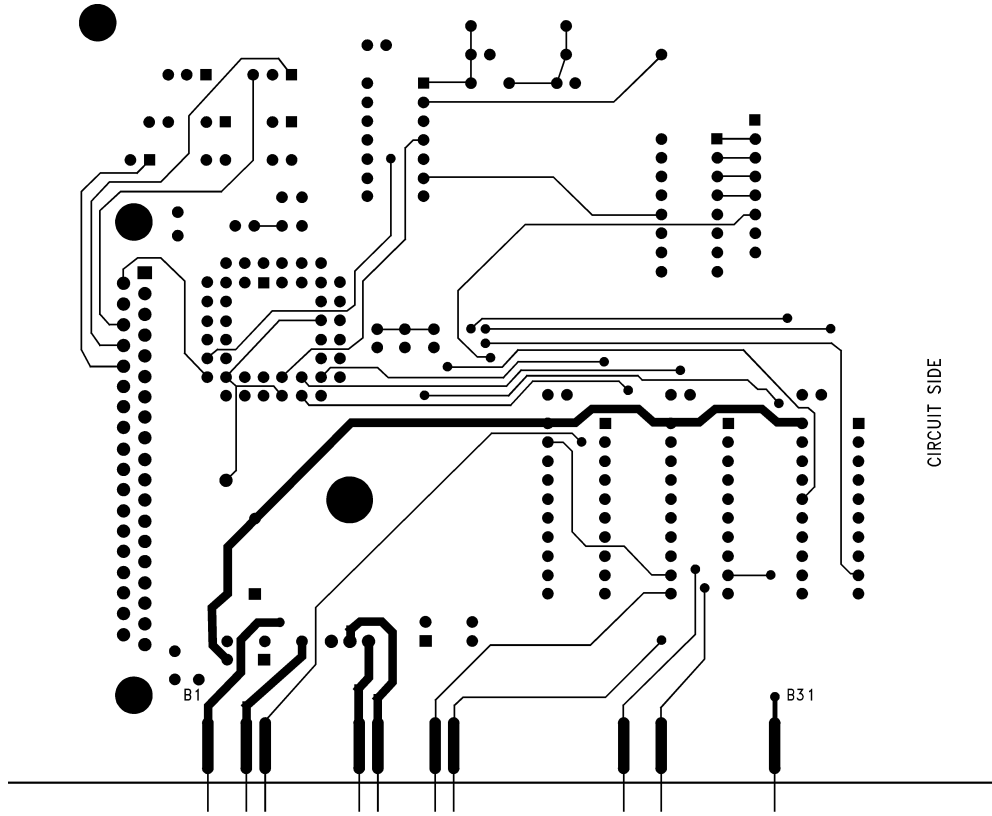
FIGURE 23. LM12(H)454/8 Evaluation/Interface Circuit-Side Layout Positive
