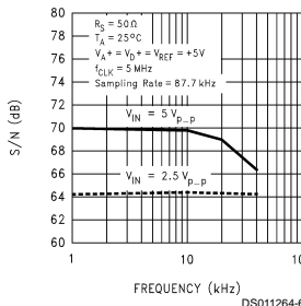
Unipolar Signal-to-Noise Ratio vs Input Frequency
