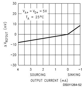
V REFOUT Load Regulation
