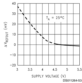
V REFOUT Line Regulation
