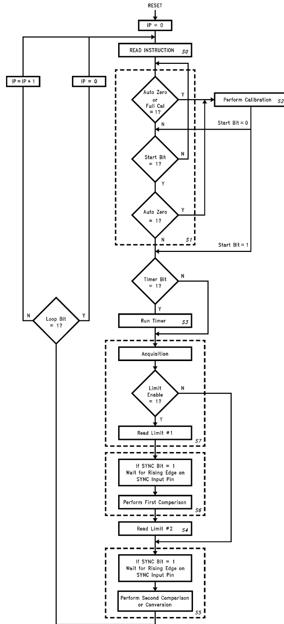
FIGURE 15. Sequencer Logic Flow Chart (IP = Instruction Pointer)
