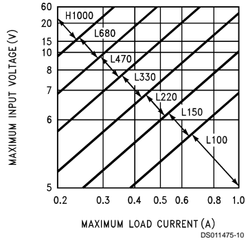
FIGURE 3. LM2575(HV)-3.3
