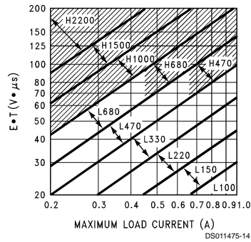
FIGURE 7. LM2575(HV)-ADJ
