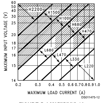
FIGURE 5. LM2575(HV)-12
