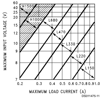
FIGURE 4. LM2575(HV)-5.0
