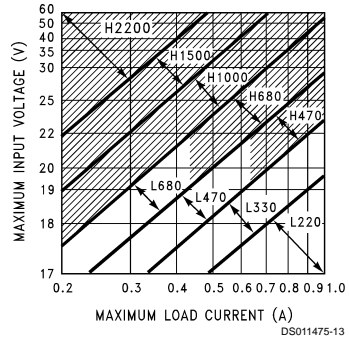
FIGURE 6. LM2575(HV)-15
