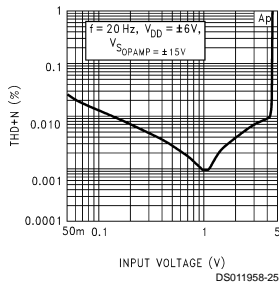
THD + N vs Amplitude f = 20 \text{ Hz} , V_{DD} = \pm 6\text{V} V_{IN} into CH1 @ 0 dB
