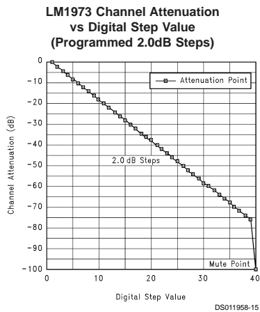
FIGURE 5. LM1973 2.0dB Attenuation Step Scheme
