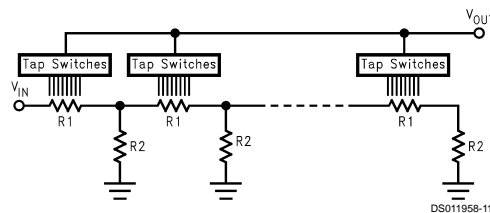
FIGURE 8. μPot Ladder Architecture
