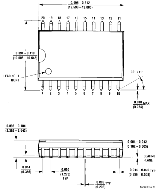
Surface Mount Package Order Number LM1973M NS Package Number M20B
