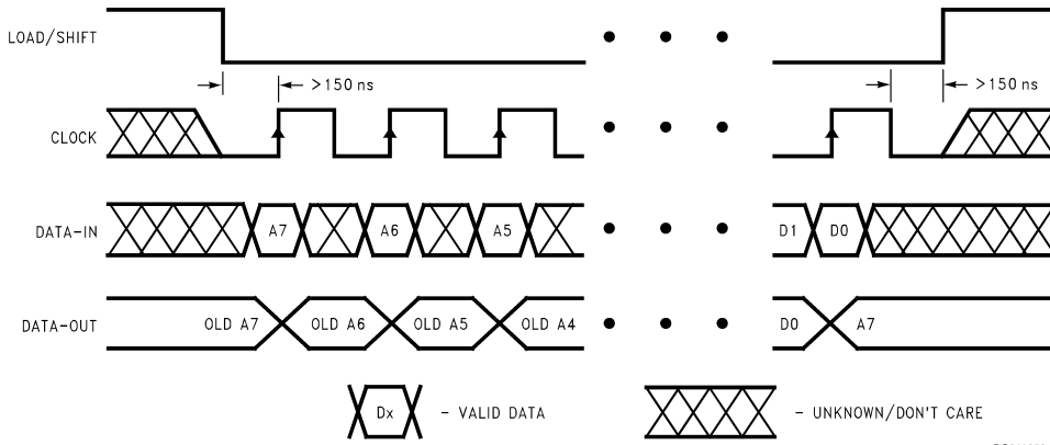
FIGURE 2. Timing Diagram
