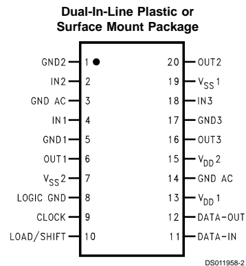
Top View Order Number LM1973M or LM1973N See NS Package Number M20B or N20A
