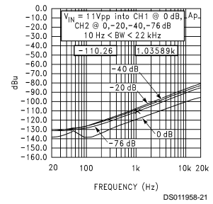
Crosstalk Test
