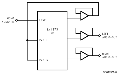
FIGURE 6. Mono Level Control with Panning Circuit
