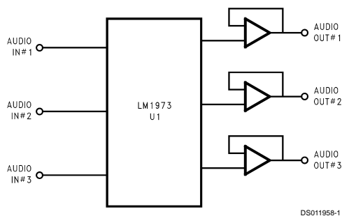
FIGURE 1. Typical Audio Attenuator Application Circuit
