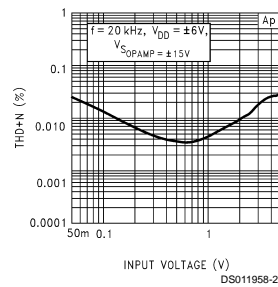
THD + N vs Amplitude f = 20 \text{ kHz} , V_{DD} = \pm 6\text{V} V_{IN} into CH1 @ 0 dB
