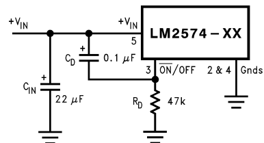
FIGURE 15. Delayed Startup
