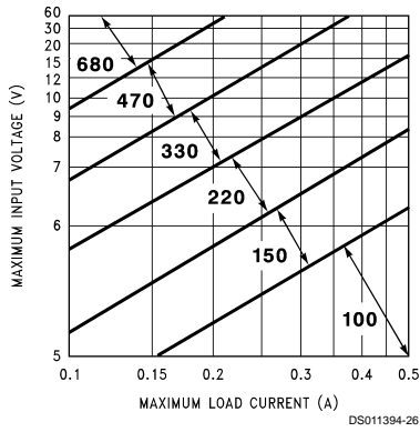
FIGURE 4. LM2574HV-3.3 Inductor Selection Guide
