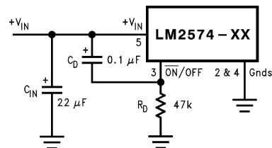
FIGURE 15. Delayed Startup
