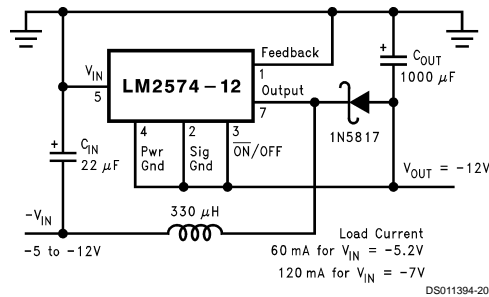
FIGURE 12. Negative Boost
