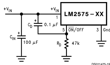
FIGURE 14. Delayed Startup
