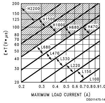
FIGURE 7. LM2575(HV)-ADJ
