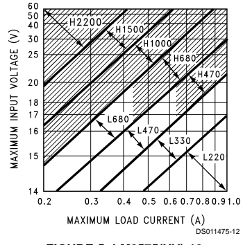
FIGURE 5. LM2575(HV)-12
