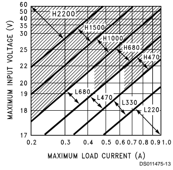
FIGURE 6. LM2575(HV)-15
